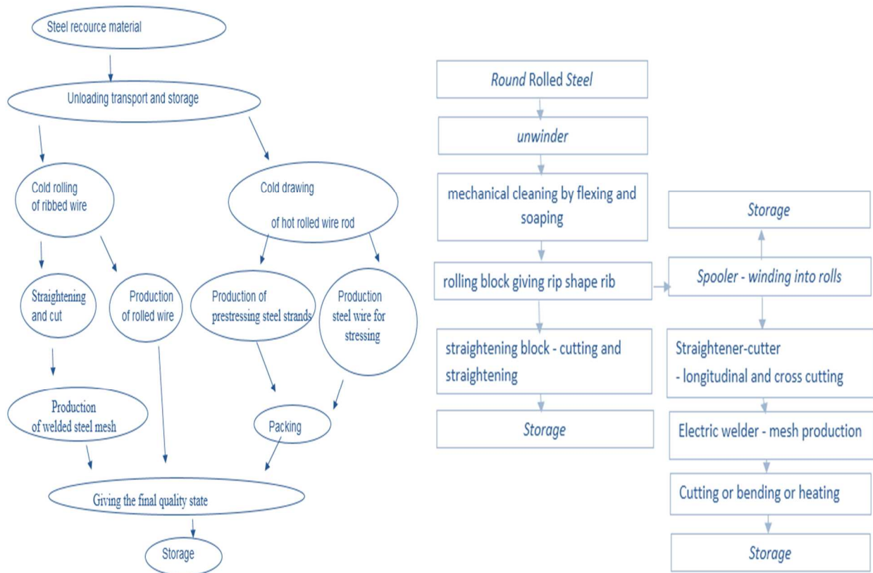
Figure 1. A scheme of manufacturing process of the SBN RUNOWO steel products
